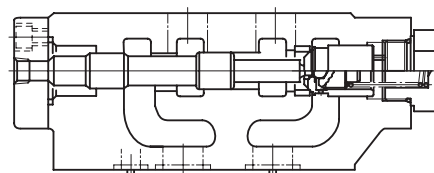
ZPB-32-*-Y-30/3090
