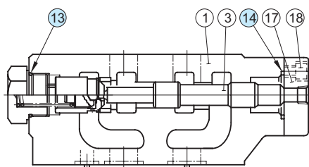
ZPA-32-*-Y-30/3090
