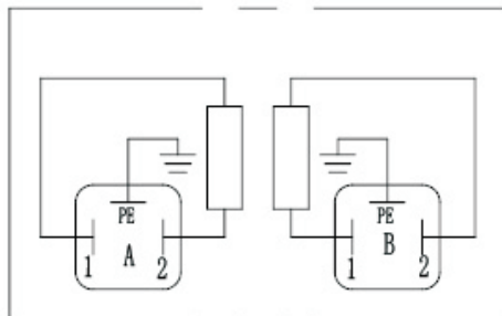
Connection at component plug
