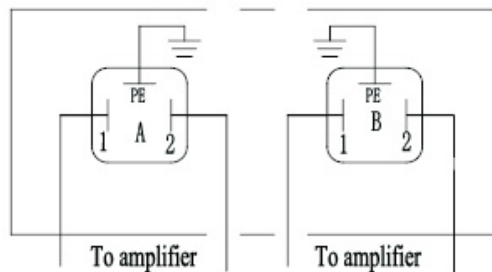
Connection at plug-in connector
