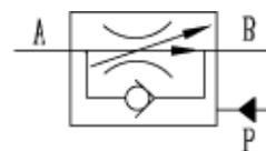
Type 2FRM6A..-20B/..R
