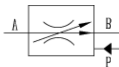
Type 2FRM6B..-20B/..M
