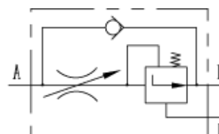
Type 2FRM6A~-20B/~M
