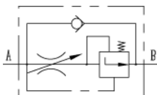
Type 2FRM6B~-20B/~M
