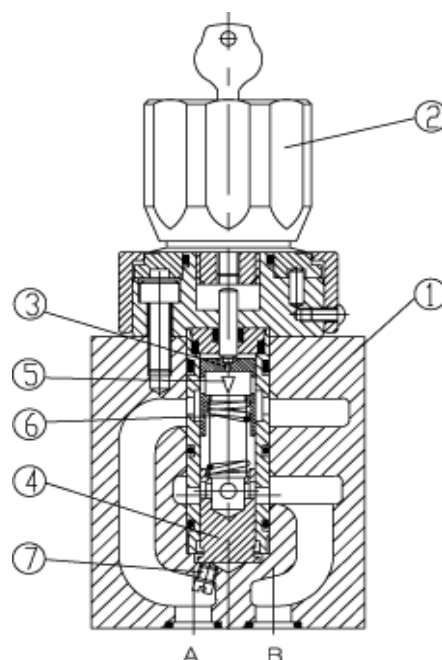
Type 2FRM6B36-20B/...M...
